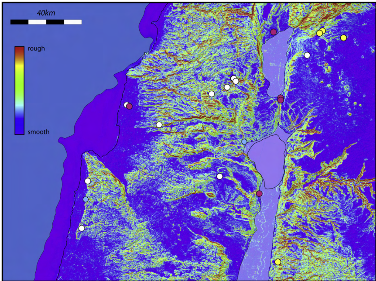
Fig. 6. Slopes and roughness in the Carmel, Galilee and Golan regions. The range of slopes that would be difficult or impossible for large herbivores to negotiate is indicated. See discussion in the text. Note that the eastern flank of the Upper Jordan valley and the western part of the Jordan plateau are heavily dissected, limiting their use even when climate was favourable. Site colours as in Figs. 1 and 2. (For interpretation of the references to colour in this figure legend, the reader is referred to the web version of this article.)
