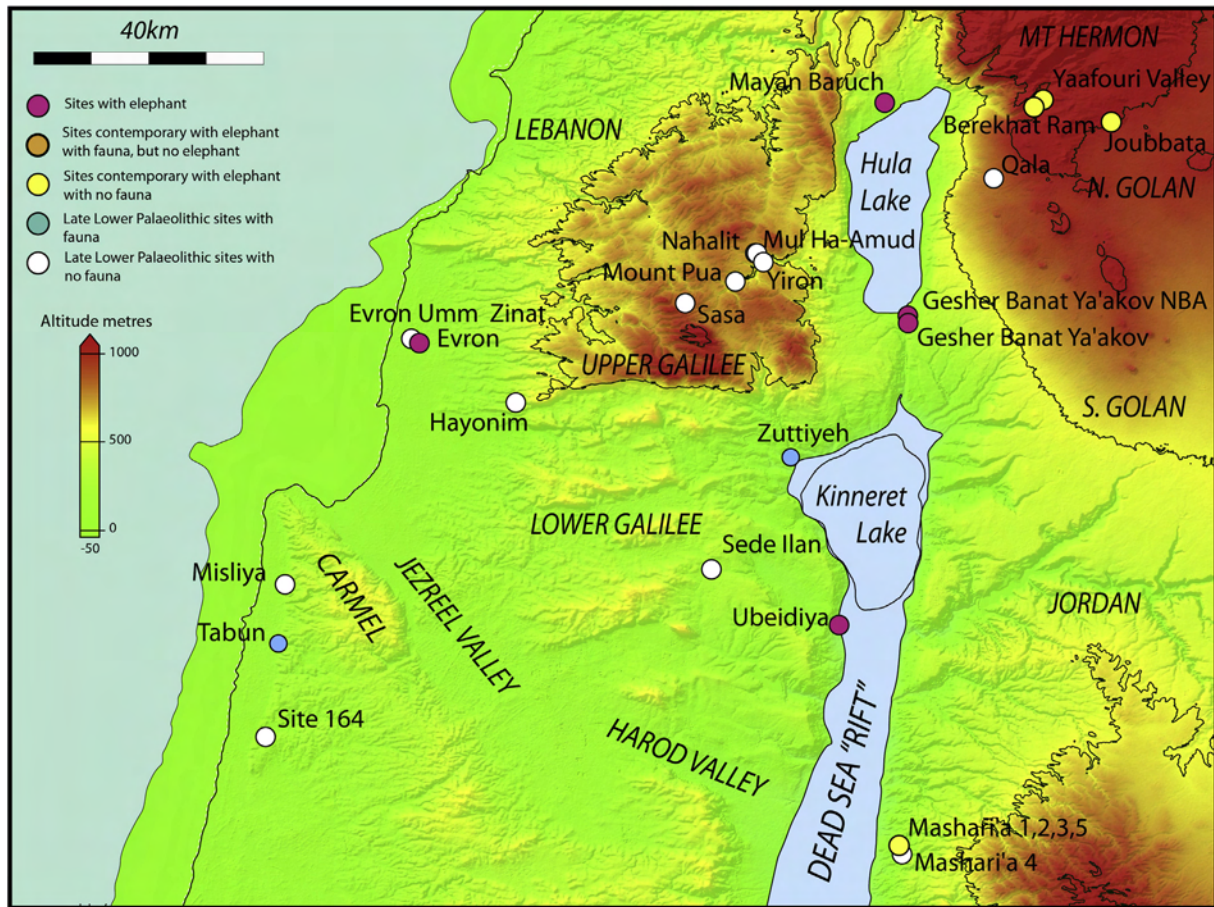
Fig. 2. The Carmel, Galilee and Golan region showing significant Lower Palaeolithic sites. The current coastline (dashed) and the coastline at -50 m are shown. Lake Lisan is shown at its maximum extent. This can be taken to approximate high levels of Lake Amora. The current Lake Kinneret is outlined. The Jordan Valley is not technically a Rift, but has many features typical of the Red Sea and East African Rifts (Devès et al., 2011). Site colours as in Fig. 1. (For interpretation of the references to colour in this figure legend, the reader is referred to the web version of this article.)
