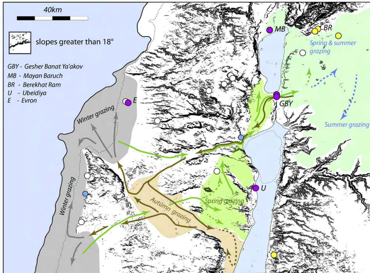
Fig. 7. Reconstructed seasonal movements of large herbivores in the middle Pleistocene of the Carmel, Galilee and Golan regions. Green arrows show suggested spring movements, blue arrows possible summer movements, and brown arrows suggested autumn movements. (For interpretation of the references to colour in this figure legend, the reader is referred to the web version of this article.)
