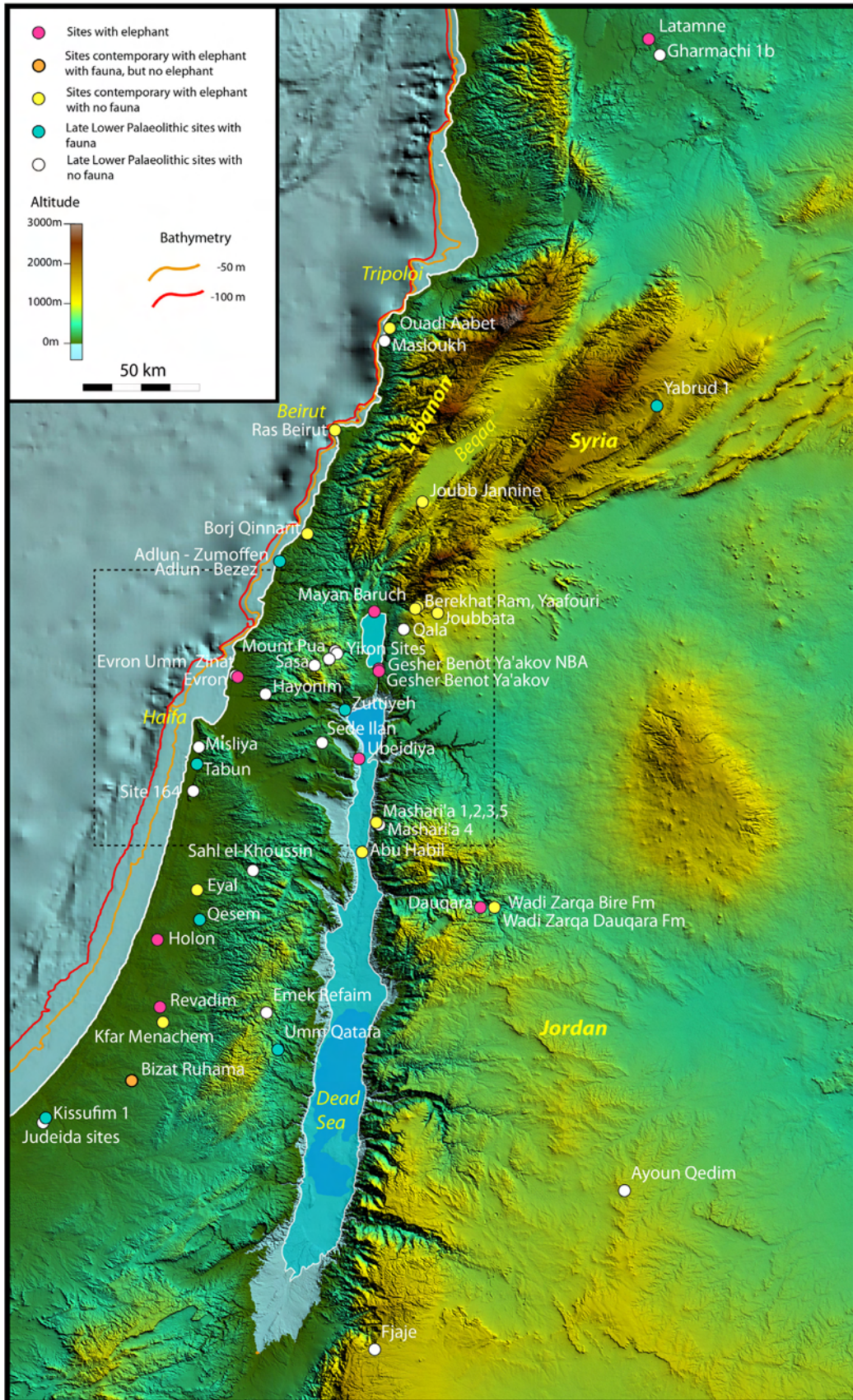
Fig. 1. Significant Lower Palaeolithic sites in the Southern Levant, plotted on to a relief map. The Late Lower Palaeolithic sites probably postdate the extinction of elephants in the region. The sea levels shown are the present-day, -50 m (orange contour) and -100 m (red contour). The current Dead Sea is shown in dark blue and Lake Lisan is shown at its maximum extent in light blue. This can be taken to approximate high levels of Lake Amora. Changing lake levels illustrate the sensitivity to climate changes. Note that the coastal plain becomes very narrow for all sea levels in what is now Lebanon restricting access to the north. Briefly sea level could have been a few metres higher than at present. A black dashed line indicates the region shown in later figures. (For interpretation of the references to colour in this figure legend, the reader is referred to the web version of this article.)
