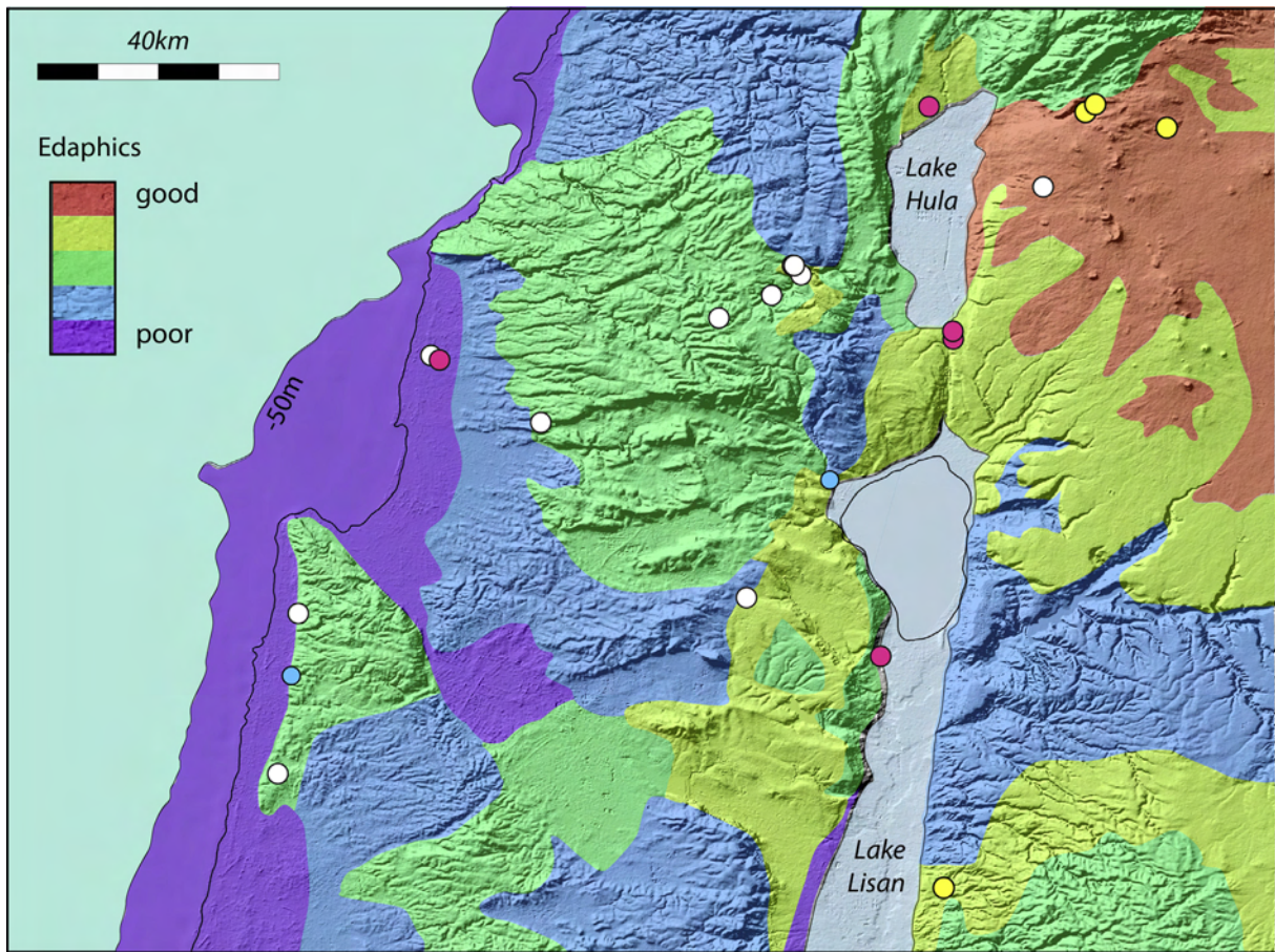
Fig. 4. Interpreted principal edaphic characteristics of the Carmel, Galilee and Golan regions, plotted on a relief map. Edaphic characteristics are based on the geology. Site colours as in Figs. 1 and 2. (For interpretation of the references to colour in this figure legend, the reader is referred to the web version of this article.)
