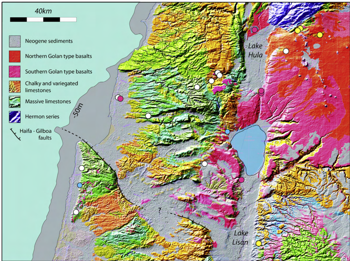
Fig. 3. Simplified geological map of the Carmel, Galilee and Golan regions, plotted on a relief map. Only the Haifa and Gilboa faults are shown. It is the modest, but ongoing motion on these faults that maintains marshy conditions in the Jezreel and Harod valleys. The morphology of the region is dominated by faulting that has occurred over the last 5 Myr and longer. More information is provided by references in the text. Site colours as in Figs. 1 and 2. The map is modified from the Geological Map of Israel, 1:200,000, State of Israel, Ministry of National Infrastructures, Geological Survey of Israel, Jerusalem 1998. (For interpretation of the references to colour in this figure legend, the reader is referred to the web version of this article.)
