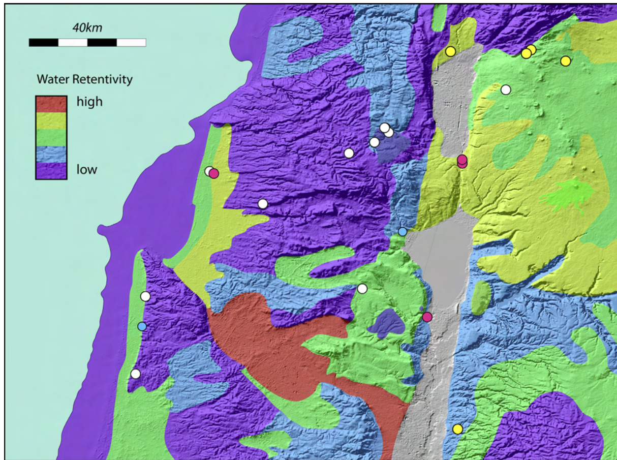
Fig. 5. Simplified map of relative water retentivity of soils in the Carmel, Galilee and Golan regions. Typical soil thickness as well as water retentivity are used to construct the figure. Sea level in this figure is shown at -50 m. Site colours as in Figs. 1 and 2. (For interpretation of the references to colour in this figure legend, the reader is referred to the web version of this article.)
