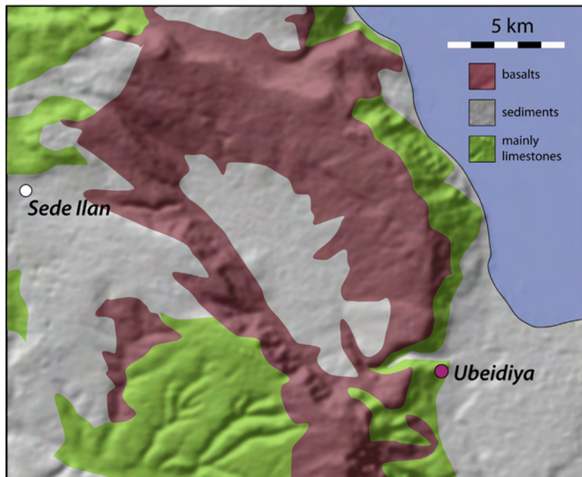
Fig. 9. The location of 'Ubeidiya in relation to prime grazing areas to the west of the site. While the detailed topography local to the site has changed very considerably, the larger-scale relationship of the site location to the landforms, rock formations and sediments to the west is essentially unchanged in the last 1.4 Myr. Note that at lower lake levels when access was possible to the east flank of the Jordan valley, the rough topography limited its usefulness (see Figs. 6 and 7).
