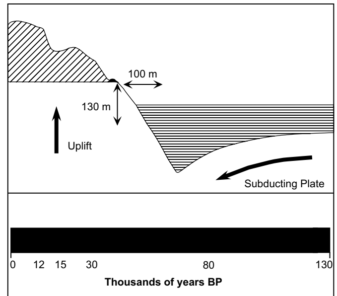
Fig. 6. Window of visibility for shell mounds on a subducting coastline. Conventions are as in previous figures. Subduction may be associated with uplift as in Fig. 5.
