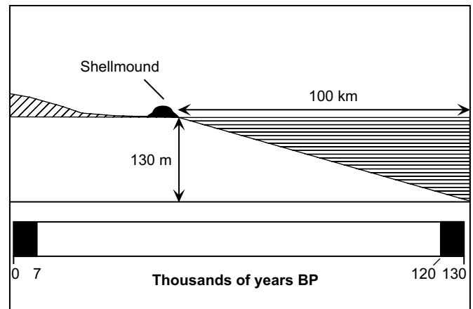
Fig. 2. Window of visibility above sea level for shell mounds adjacent to a shallow shelf. Black = visible, white = invisible. Shell mounds or other coastal sites with marine resources are expected to be visible only at highest sea levels, those associated with lower sea levels to be submerged.
