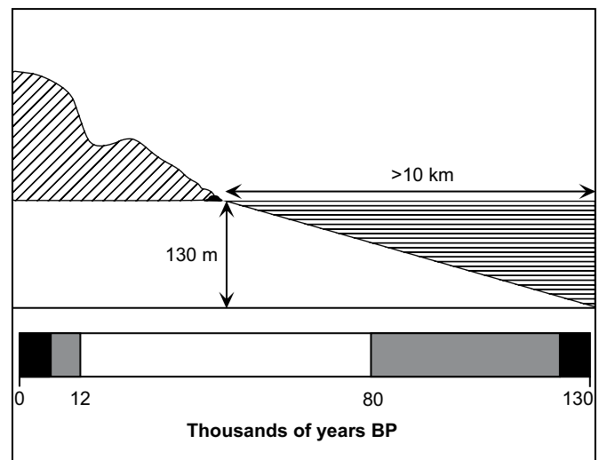
Fig. 3. Window of visibility for shell mounds near a narrower shelf. Conventions are as in Fig. 1. Gray = some marine resources visible in deposits on present-day land and some deposited in now-submerged locations.
