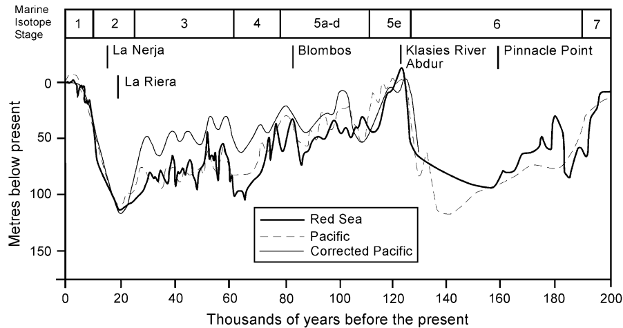
Fig. 1. Simplified sea-level curves for the past 200 ka, showing archaeological sites with evidence of marine resources (see text for further details). The Red Sea and Pacific records are derived from \delta^{18}\text{O} measurements of benthic foraminifera. The corrected record is based on corrections derived from elevated coral terraces. Sources: Chappell and Shackleton, 1986; Shackleton, 1987; Imbrie et al., 1984; Lambeck and Chappell, 2001; Lambeck et al., 2002; Waelbroeck et al., 2002; Siddall et al., 2003; Antonioli et al., 2004.
