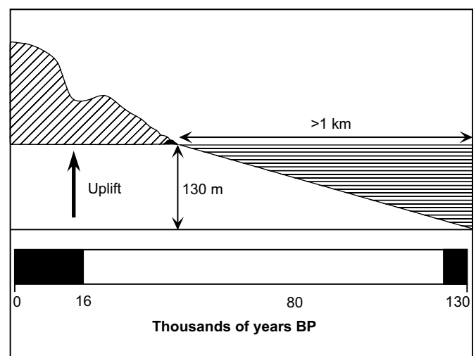
Fig. 5. Window of visibility for shell mounds on a coastline uplifted by isostatic or tectonic movement. The duration of the window depends on the amount of uplift of the coastal site since its deposition. Conventions are as in Fig. 3. Theoretically sites could be visible throughout the full glacial period on coastlines with sufficiently rapid uplift, but this is rare in practice. See text for further discussion.
