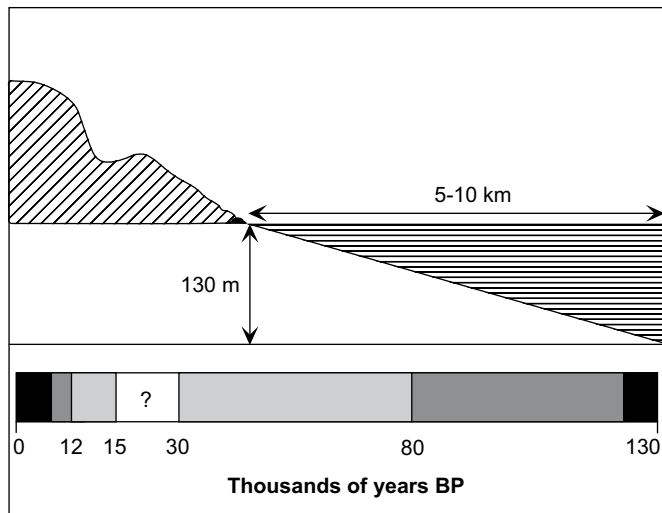
Fig. 4. Window of visibility for shell mounds near a very narrow shelf. Conventions are as in Figs. 2 and 3. Lightest gray = only minor evidence of marine resources visible on present-day land and most deposited in now-submerged locations. The duration of the window depends on the width of the shelf but is expected to be largely closed at lowest sea levels during the glacial maximum.
